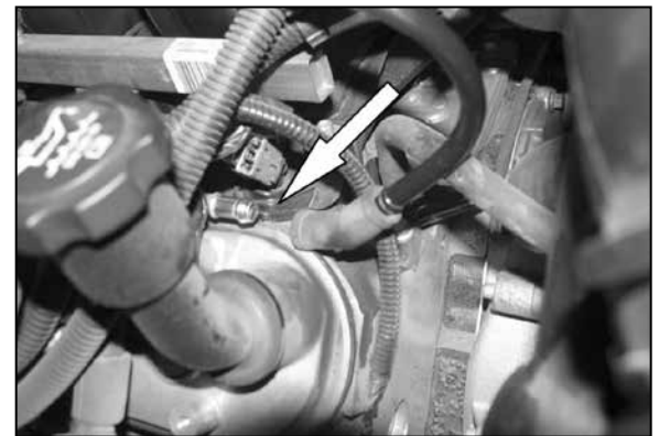
5. Disconnect crankcase vent hose from the valve cover as shown.
