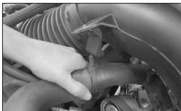
4. Unhook the radiator hose mount from the intake tube.
